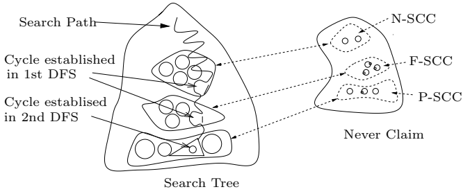
Fig. 12. Visualization of the different cases in Improved-Nested-DFS.
