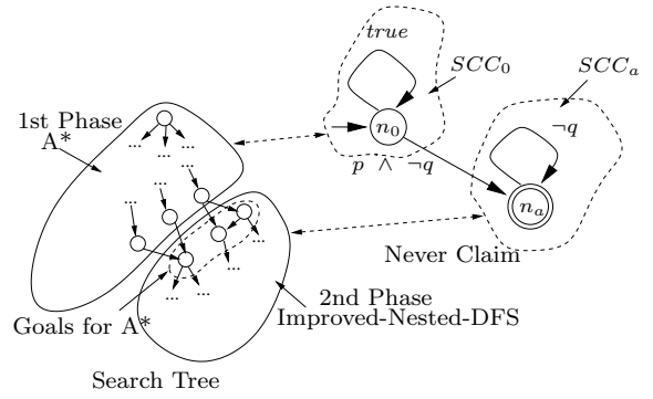
Fig. 14. Visualization of A^* and Improved-Nested-DFS for a response property.
