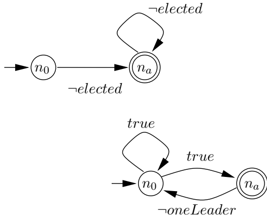
Fig. 15. Never claims for \diamond\Box oneLeader (top-left) and \diamond elected (bottom-right).
