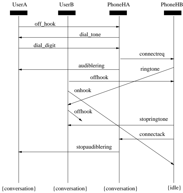
Fig. 11. POTS example, error trail generated by HSF SPIN using A^* and H_f .
